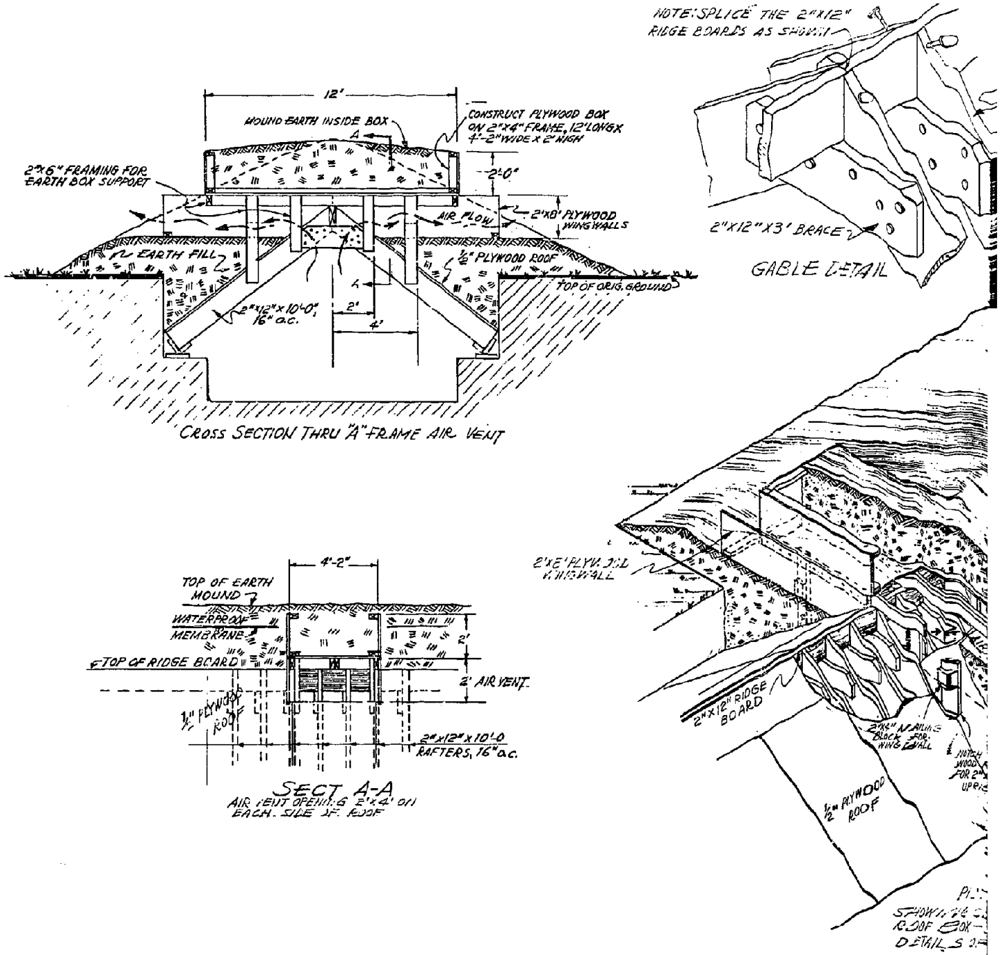
Fig. A-10.2. A-Frame Expedient Shelter, Alternate Air Vent Design.
